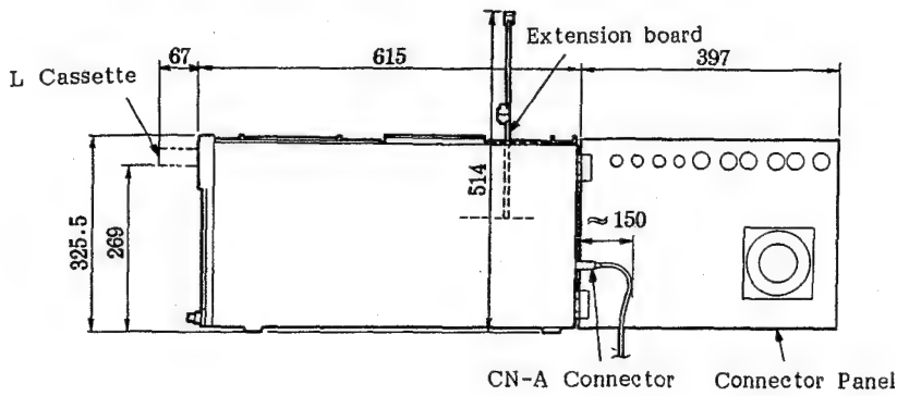
(3) Working Space: When opening Connector Panel.
